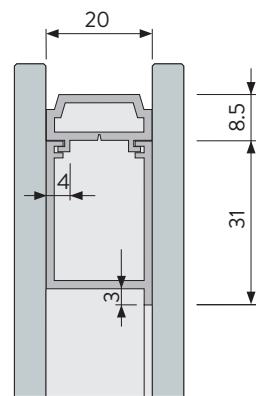
SECTION B-B
